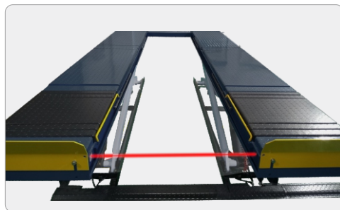
Photocell configuration for the leveling of the two platforms, more stable and safe.
