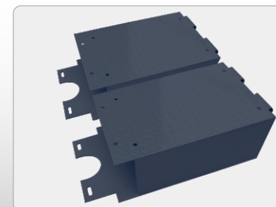
Optional platform extension kits adds an extra 660mm length to the platform. Kits No.:41403(A465 A465A) Kits No.:41801(A480 A480A).
