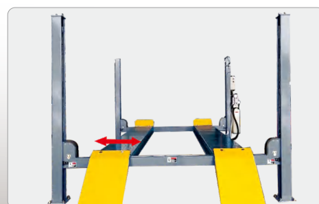
Off-side platform can be adjusted the mounting position left or right.
