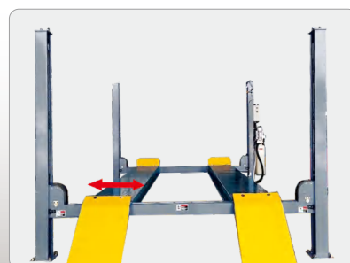
Off-side platform can be adjusted the mounting position left or right.
