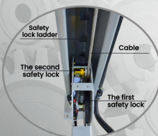
Double-safety locks
