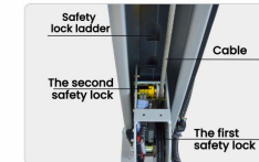
Double safety locks provide additional safety.
